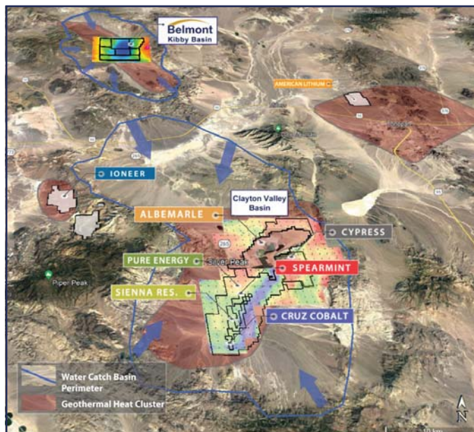
The Kibby and Clayton Valley Basins, Nevada
